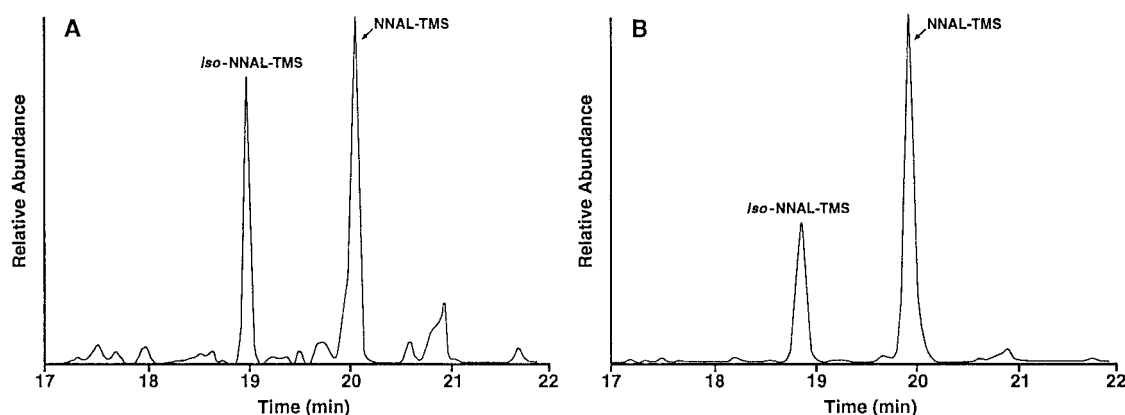
Fig. 4. Chromatograms obtained on GC-MS/MS analysis ( m/z 282→ m/z 162) of the (A) NNAL fraction and (B) NNAL-Gluc fraction of a child's urine. TMS, trimethylsilyl ether
