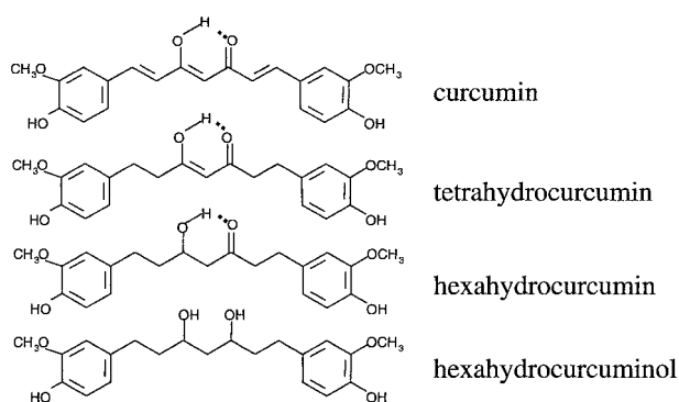
Fig. 1. Chemical structures of curcumin and products of its bioreduction.
