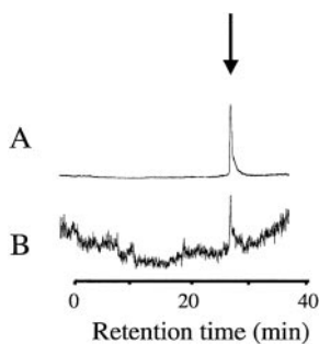
Fig. 3. On-line HPLC-mass spectrometry analysis in selected ion registration mode of curcumin sulfate (molecular ion at m/z = 447 ) derived from extracts of incubations of curcumin with human intestinal cytosol (A) and recombinant SULT1A1 (B). Arrow, retention time of authentic curcumin sulfate. For details of incubation, extraction, and HPLC analysis, see "Materials and Methods." The chromatograms are representative of analyses conducted with cytosol from 2 humans and two enzyme preparations each.
